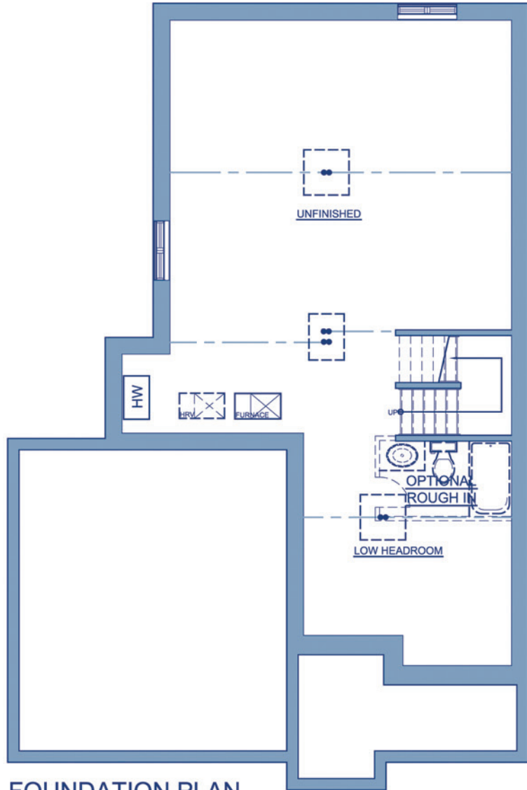
FOUNDATION PLAN
