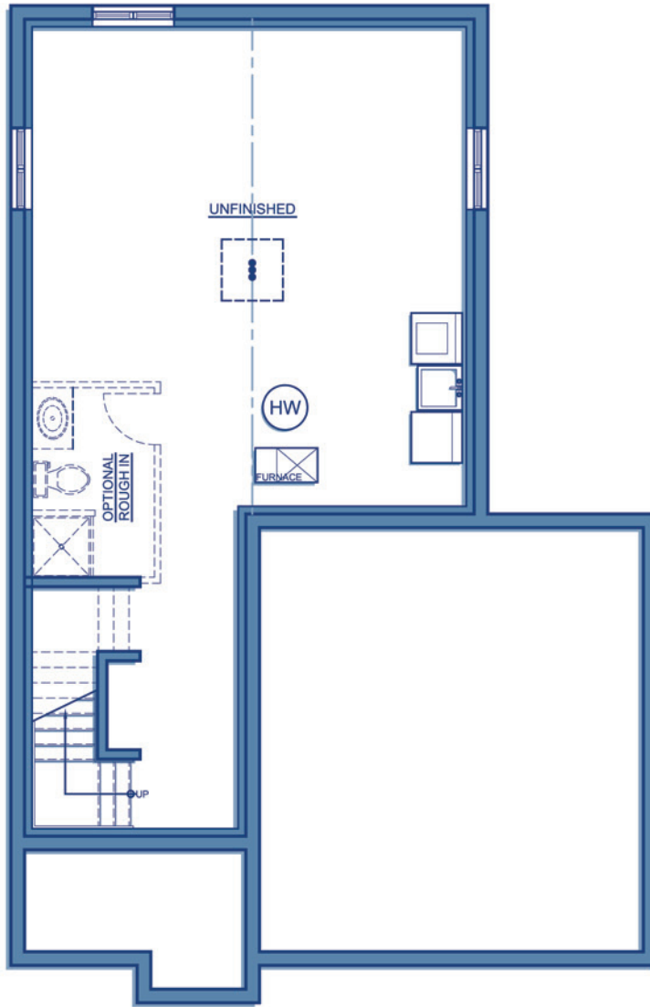
FOUNDATION PLAN
