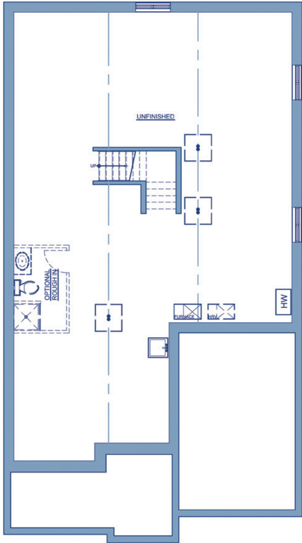
FOUNDATION PLAN
