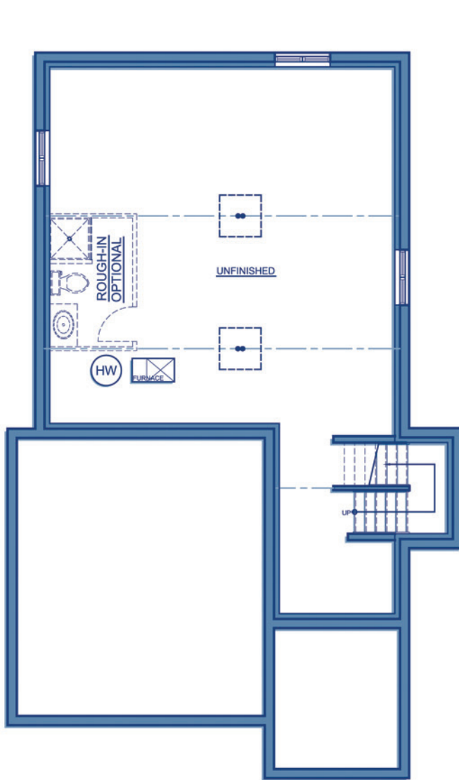
FOUNDATION PLAN
