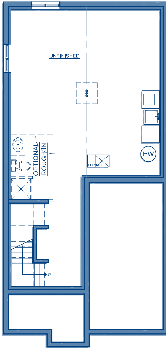
FOUNDATION PLAN
