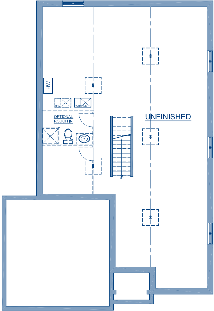
FOUNDATION PLAN
