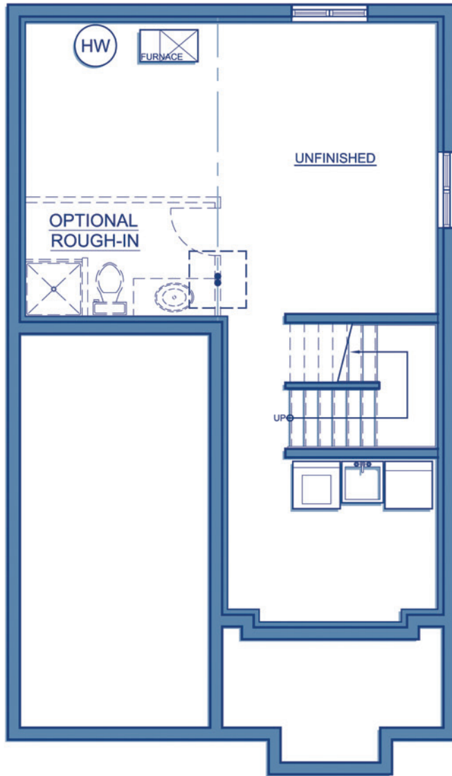
FOUNDATION PLAN
