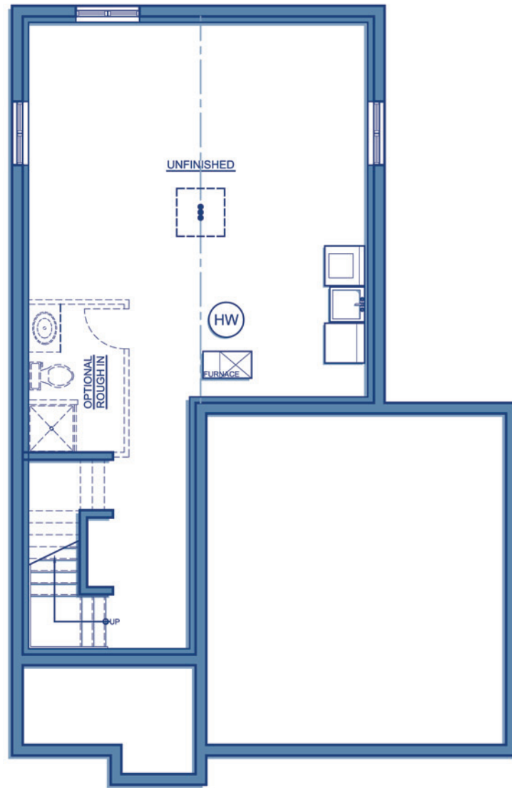
FOUNDATION PLAN
