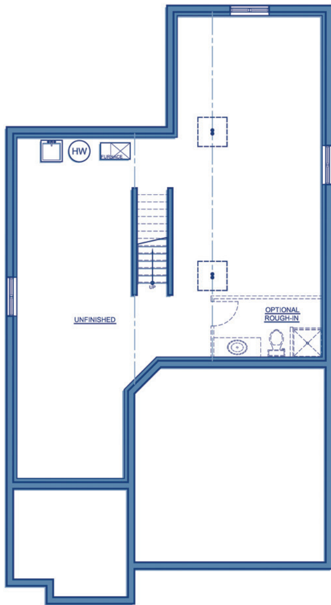
FOUNDATION PLAN
